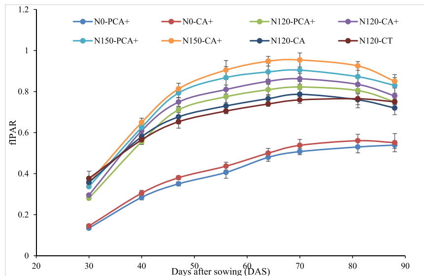
Fig. 4. Effect of different tillage, nitrogen doses and residue and irrigation management on fractional intercepted photosynthetically active radiation (fIPAR) of maize. Vertical bars are standard error (SE) within each treatment. *Refer to Table 1 for treatment details .
